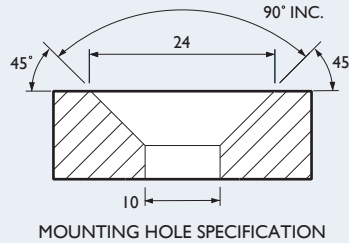
MOUNTING HOLE SPECIFICATION
